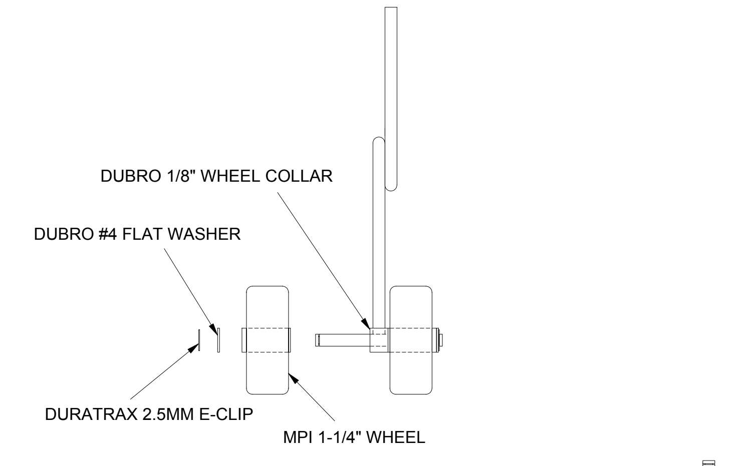
NOSE GEAR DETAIL
