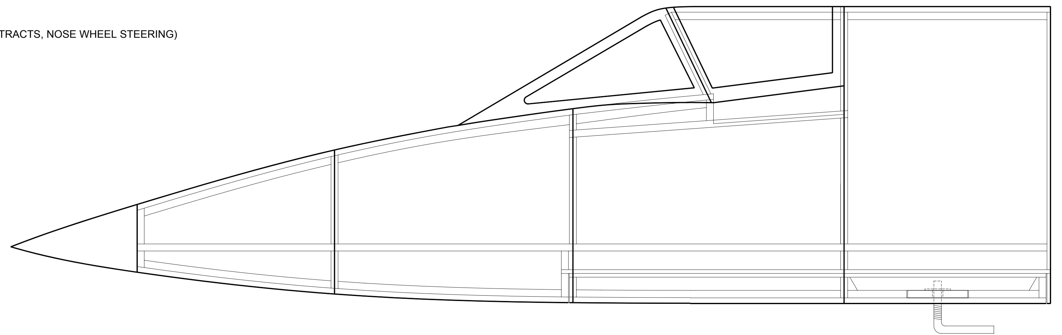
SIDE VIEW (LEFT SIDE SHEETING AND LEFT WING OMITTED FOR CLARITY)
